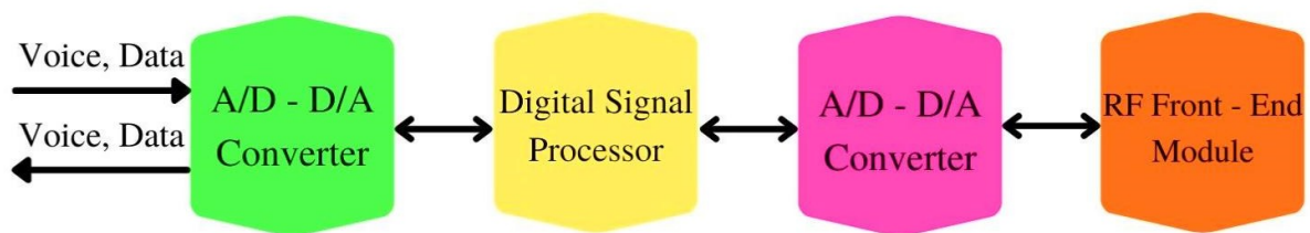
Figure 4. Software Radio Architecture that is Ideal
